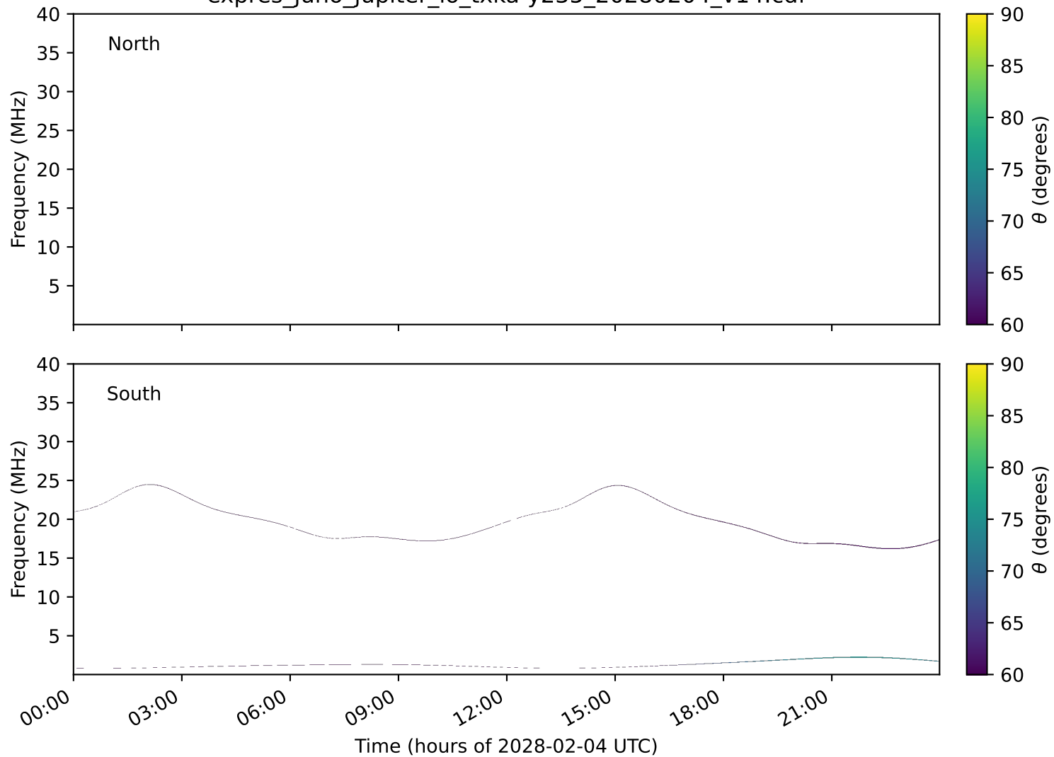
expres_juno_jupiter_io_txka-y235_20280204_v14.cdf
