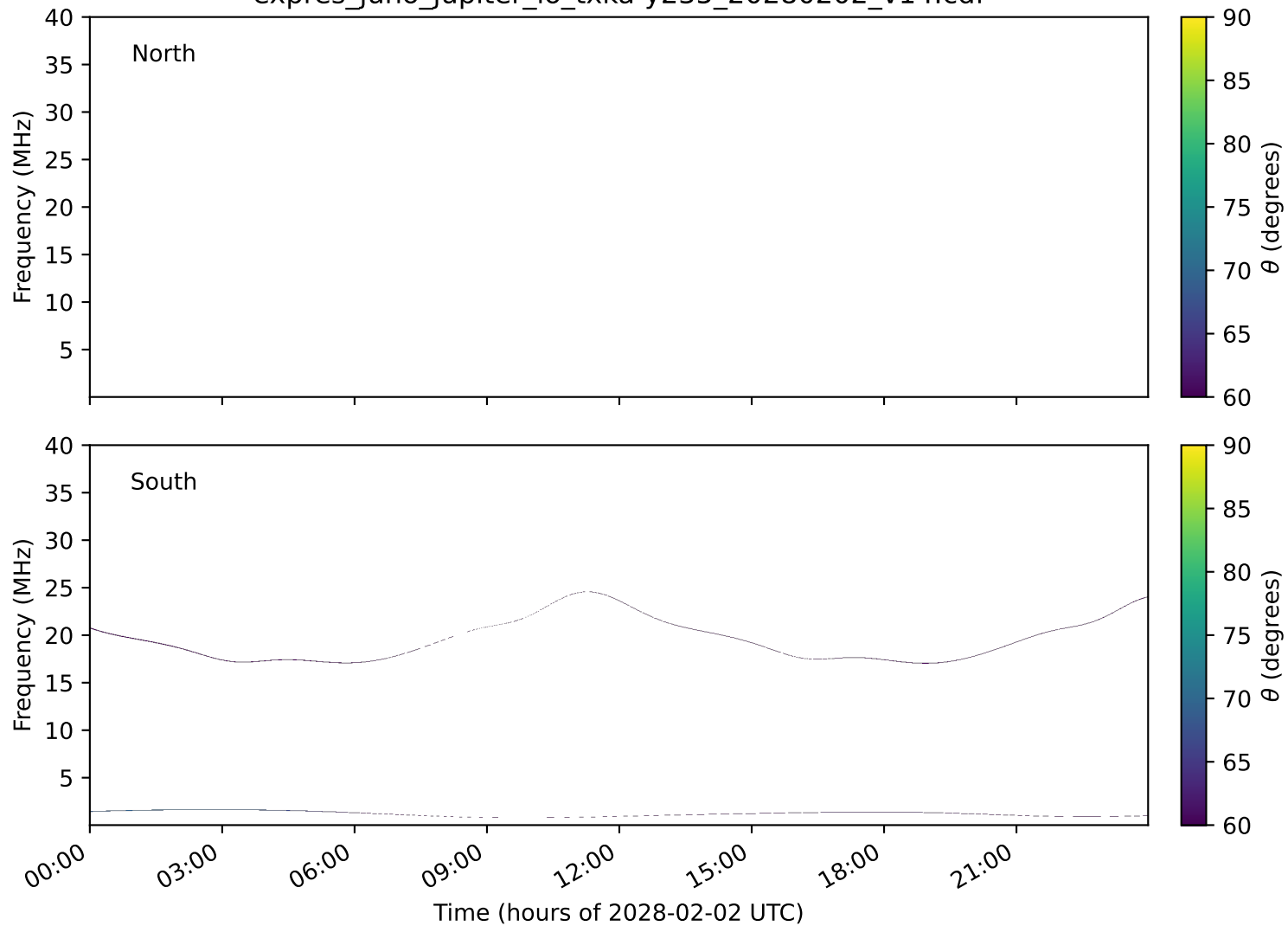
expres_juno_jupiter_io_txka-y235_20280202_v14.cdf
