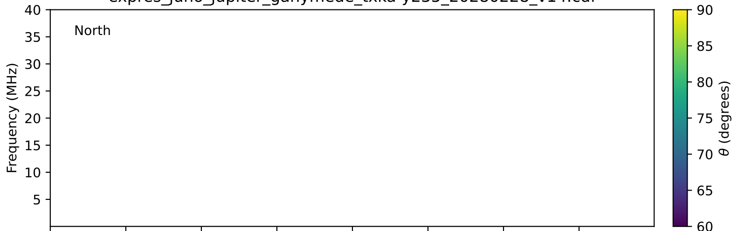
expres_juno_jupiter_ganymede_txka-y235_20280228_v14.cdf
