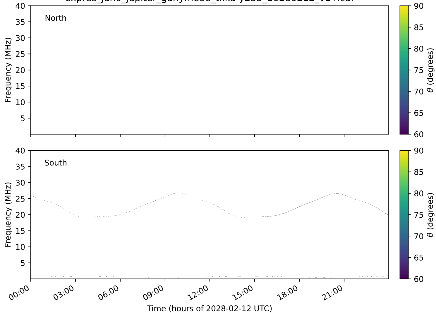
expres_juno_jupiter_ganymede_txka-y235_20280212_v14.cdf
