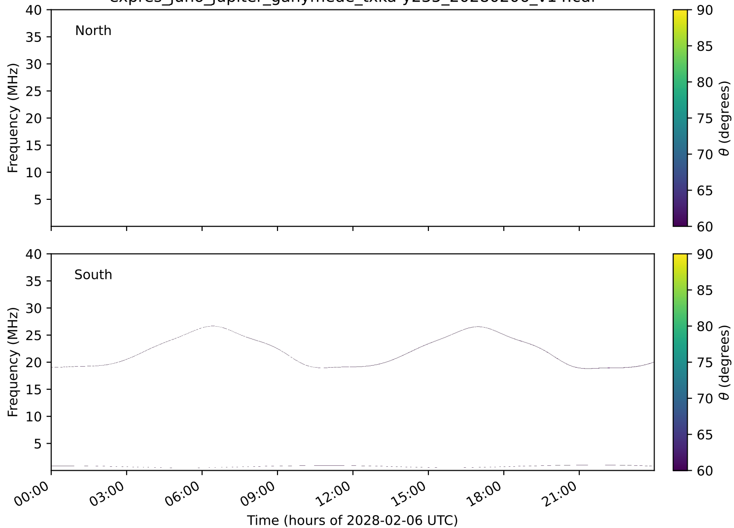
expres_juno_jupiter_ganymede_txka-y235_20280206_v14.cdf
