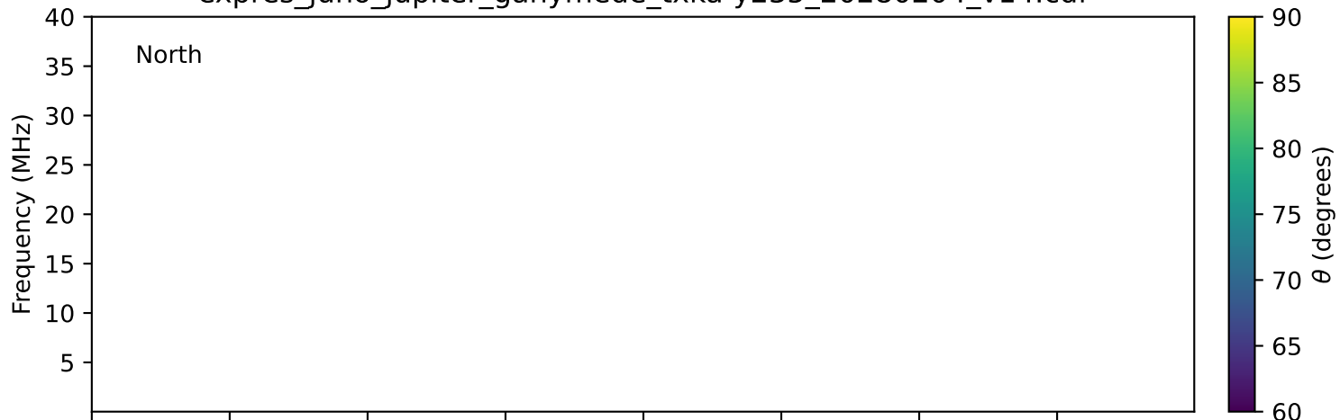
expres_juno_jupiter_ganymede_txka-y235_20280204_v14.cdf
