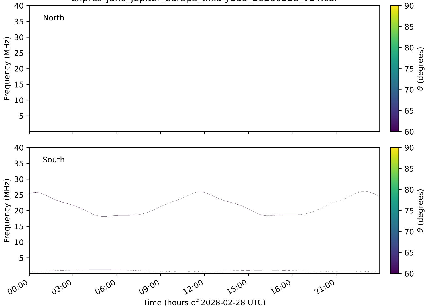
expres_juno_jupiter_europa_txka-y235_20280228_v14.cdf
