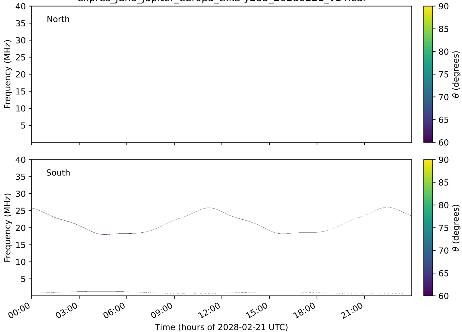
expres_juno_jupiter_europa_txka-y235_20280221_v14.cdf
