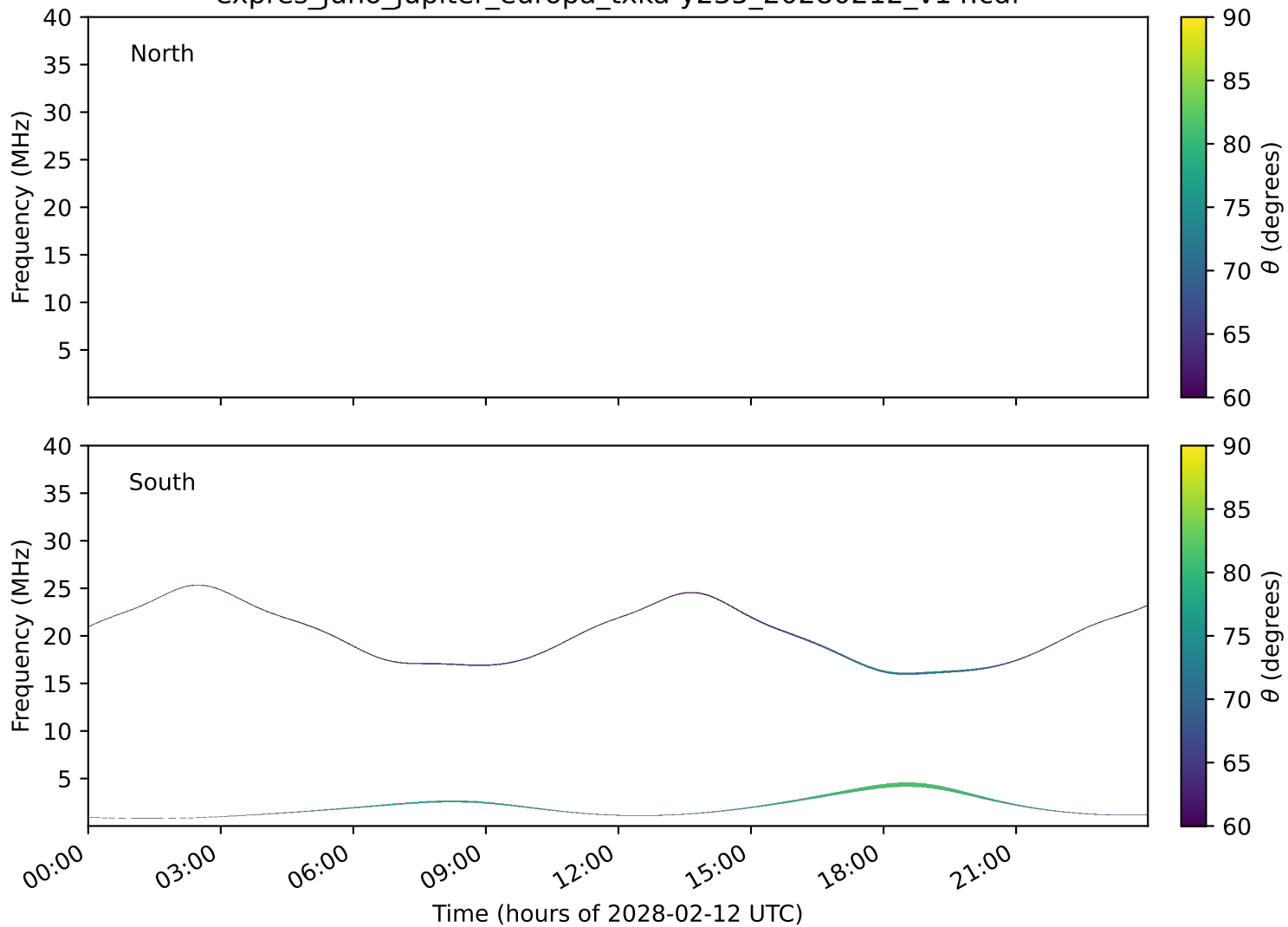
expres_juno_jupiter_europa_txka-y235_20280212_v14.cdf
