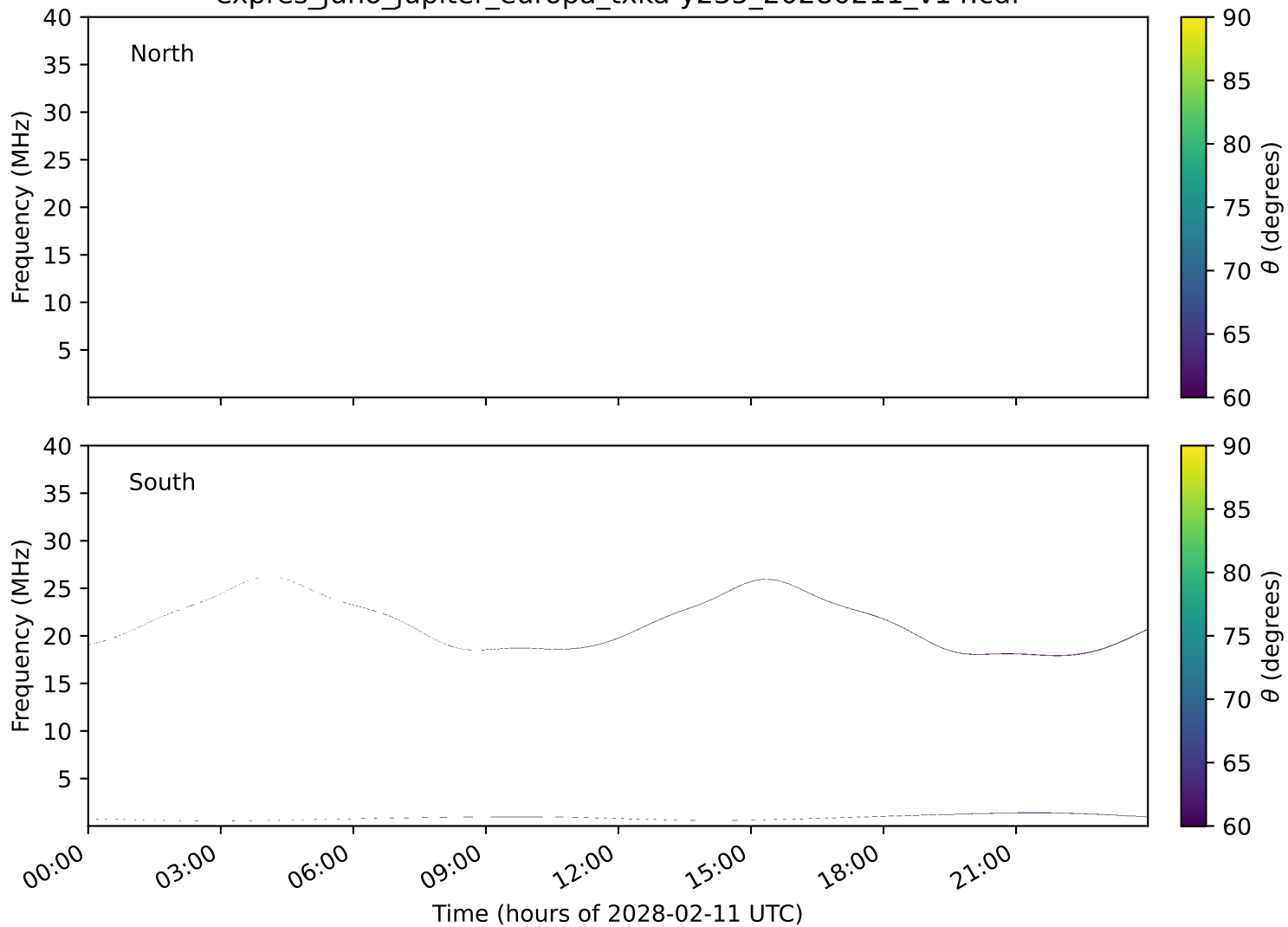
expres_juno_jupiter_europa_txka-y235_20280211_v14.cdf
