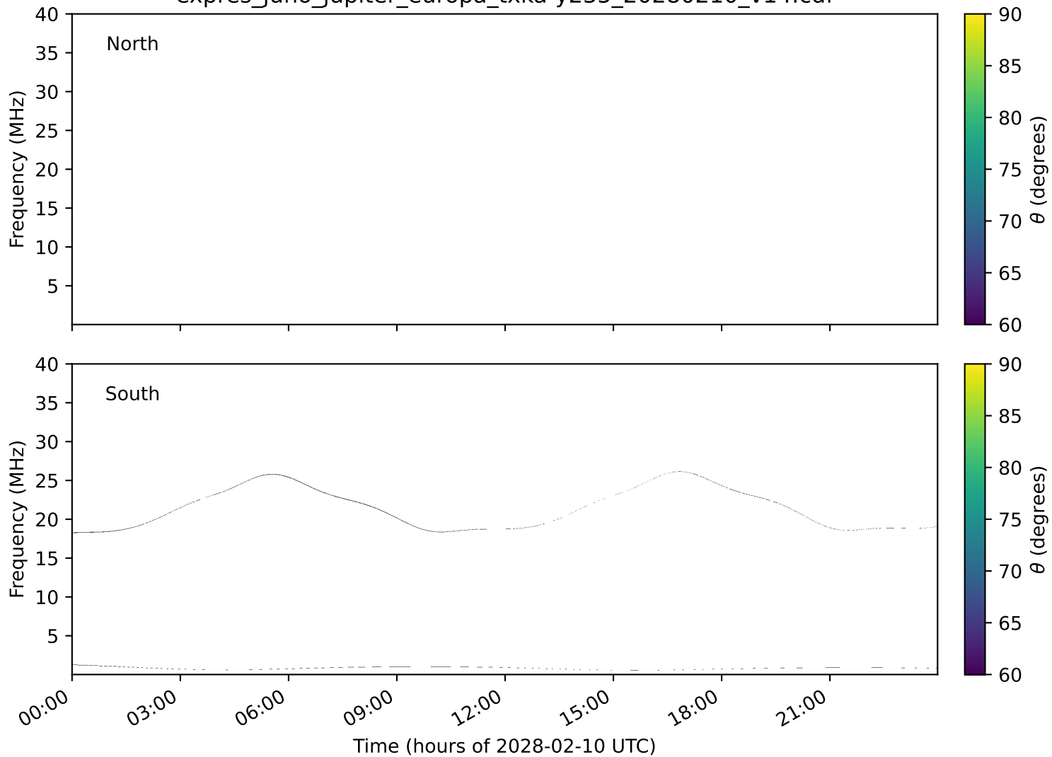
expres_juno_jupiter_europa_txka-y235_20280210_v14.cdf
