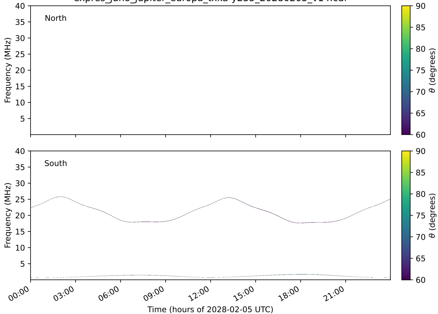
expres_juno_jupiter_europa_txka-y235_20280205_v14.cdf
