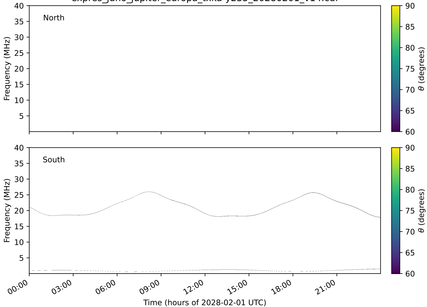
expres_juno_jupiter_europa_txka-y235_20280201_v14.cdf
