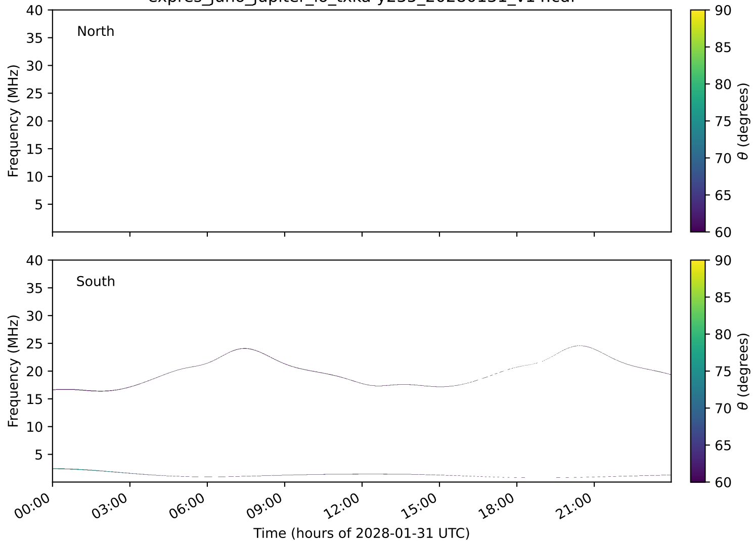
expres_juno_jupiter_io_txka-y235_20280131_v14.cdf
