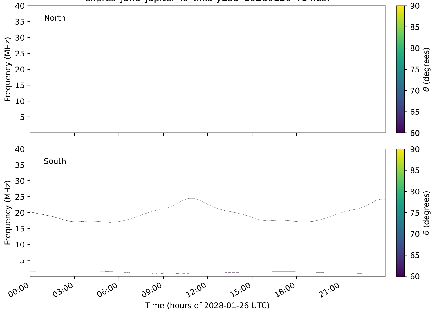
expres_juno_jupiter_io_txka-y235_20280126_v14.cdf
