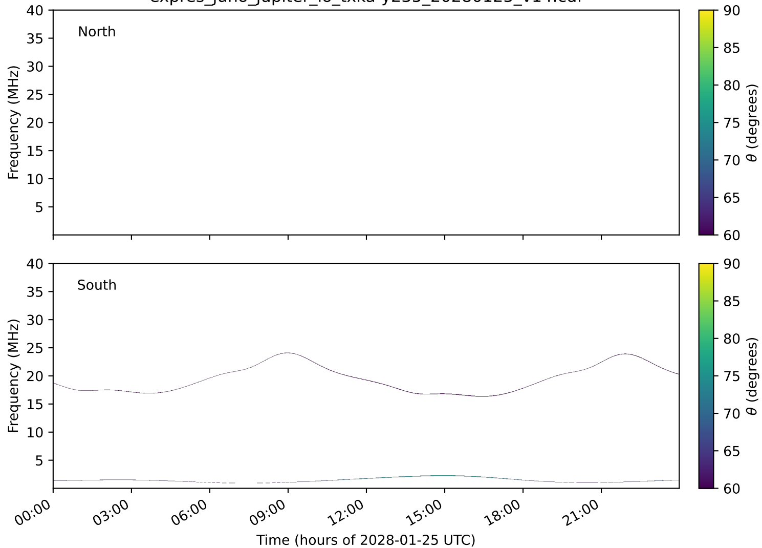
expres_juno_jupiter_io_txka-y235_20280125_v14.cdf
