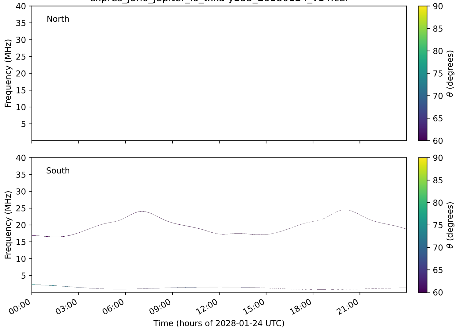
expres_juno_jupiter_io_txka-y235_20280124_v14.cdf
