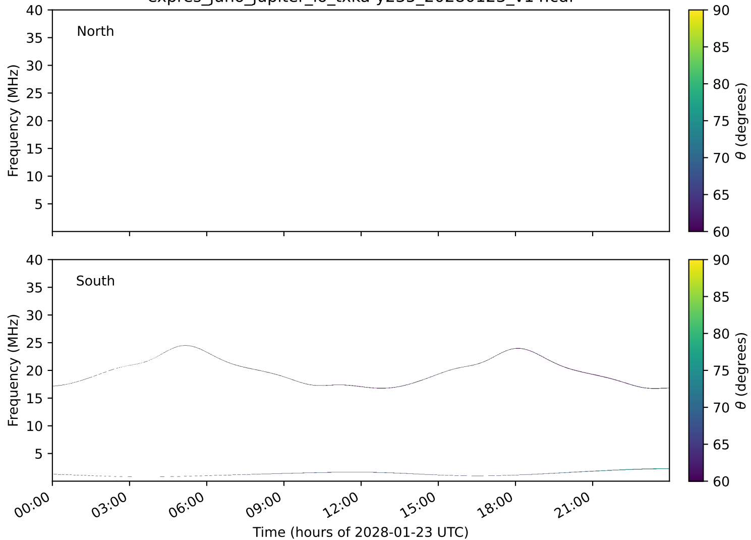
expres_juno_jupiter_io_txka-y235_20280123_v14.cdf
