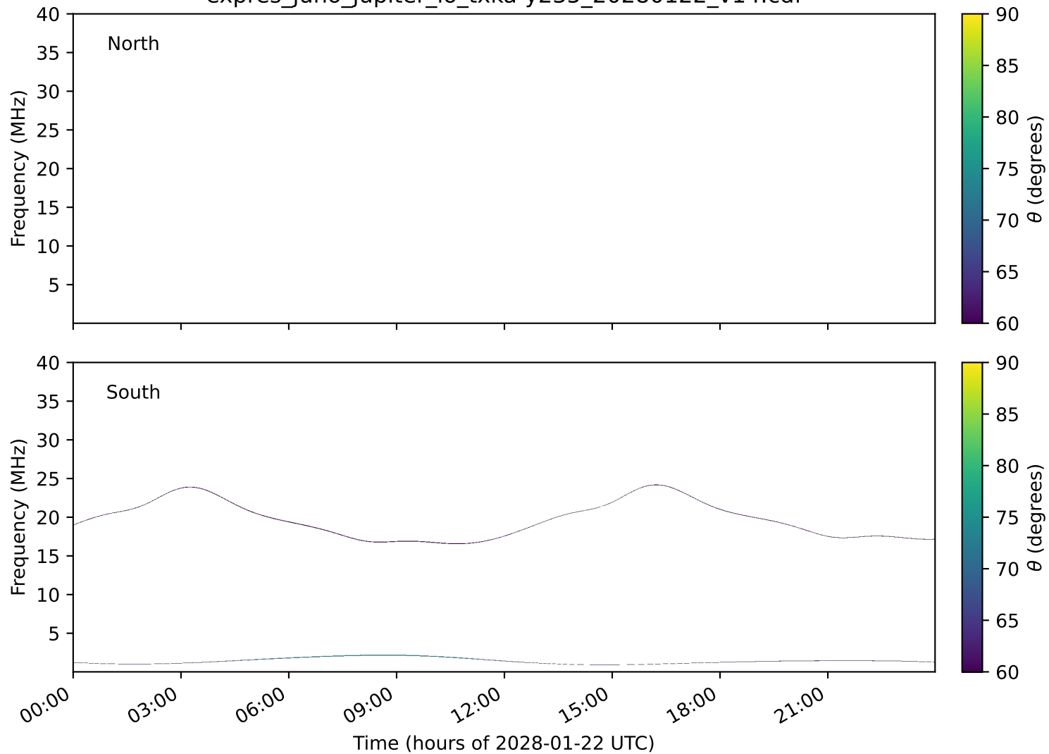
expres_juno_jupiter_io_txka-y235_20280122_v14.cdf
