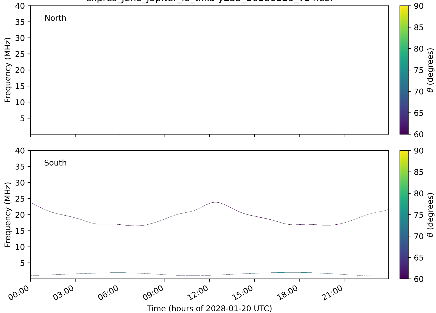
expres_juno_jupiter_io_txka-y235_20280120_v14.cdf
