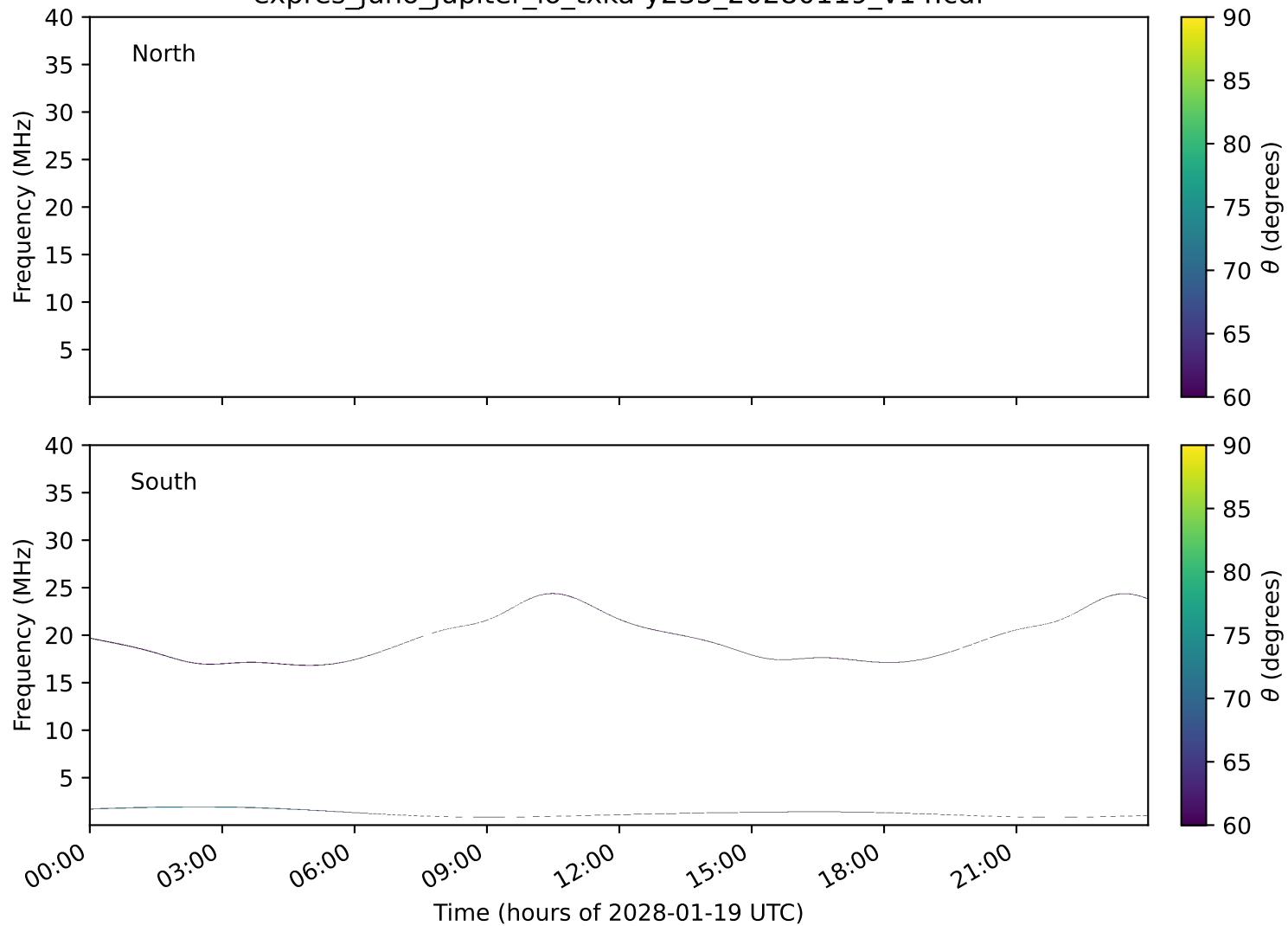
expres_juno_jupiter_io_txka-y235_20280119_v14.cdf
