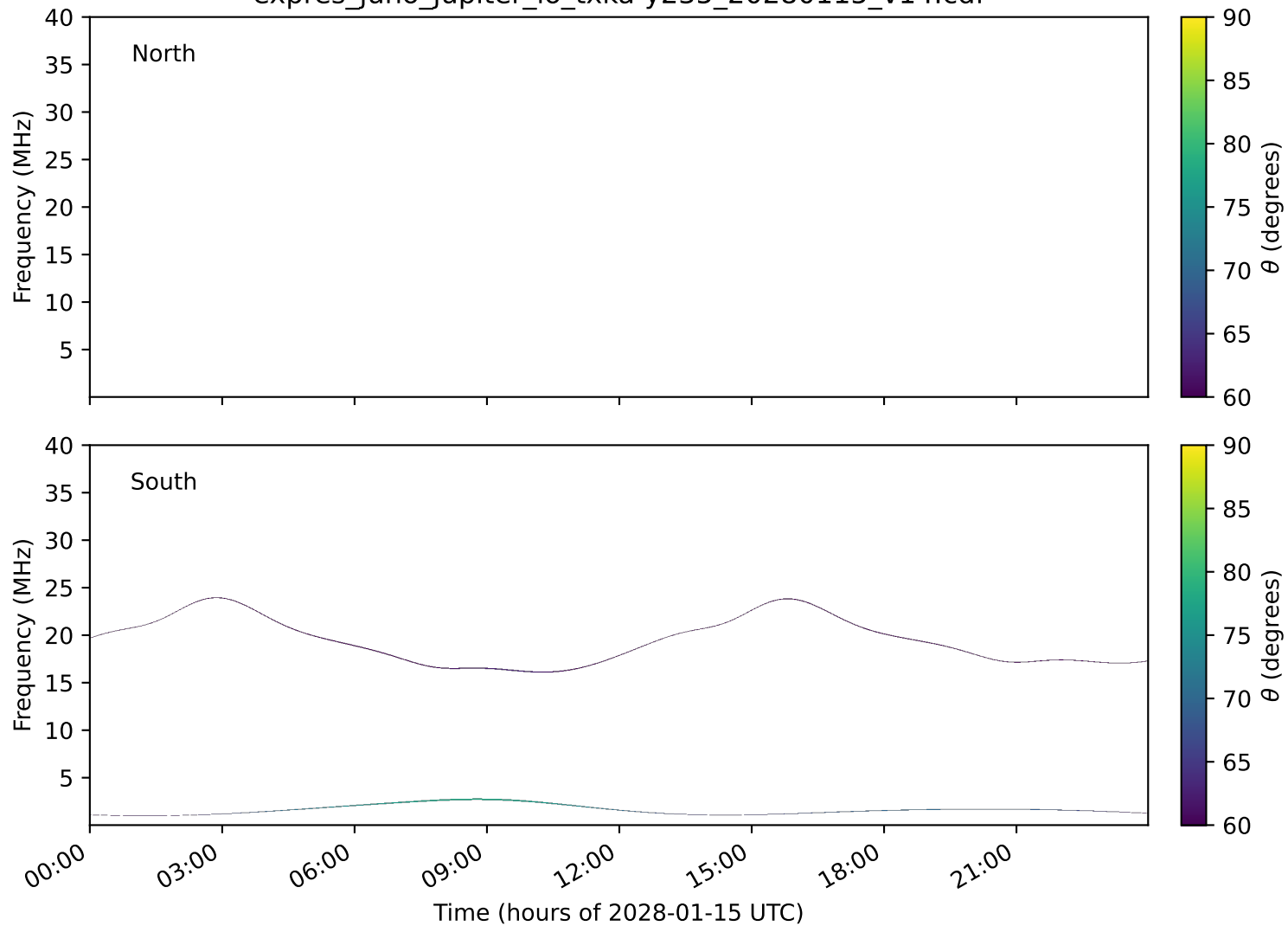
expres_juno_jupiter_io_txka-y235_20280115_v14.cdf
