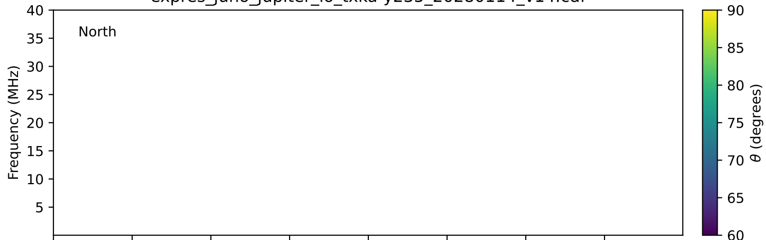
expres_juno_jupiter_io_txka-y235_20280114_v14.cdf
