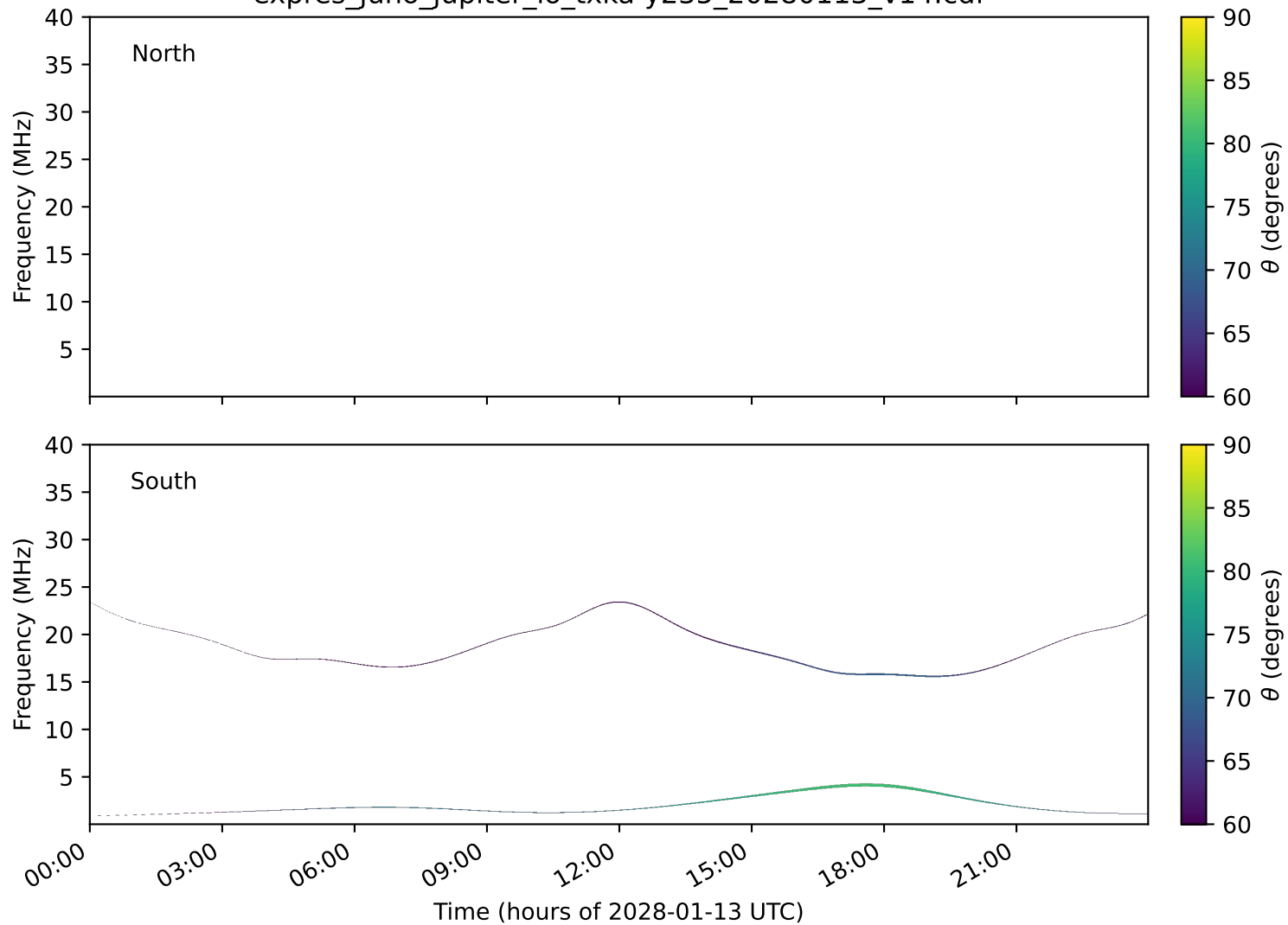
expres_juno_jupiter_io_txka-y235_20280113_v14.cdf
