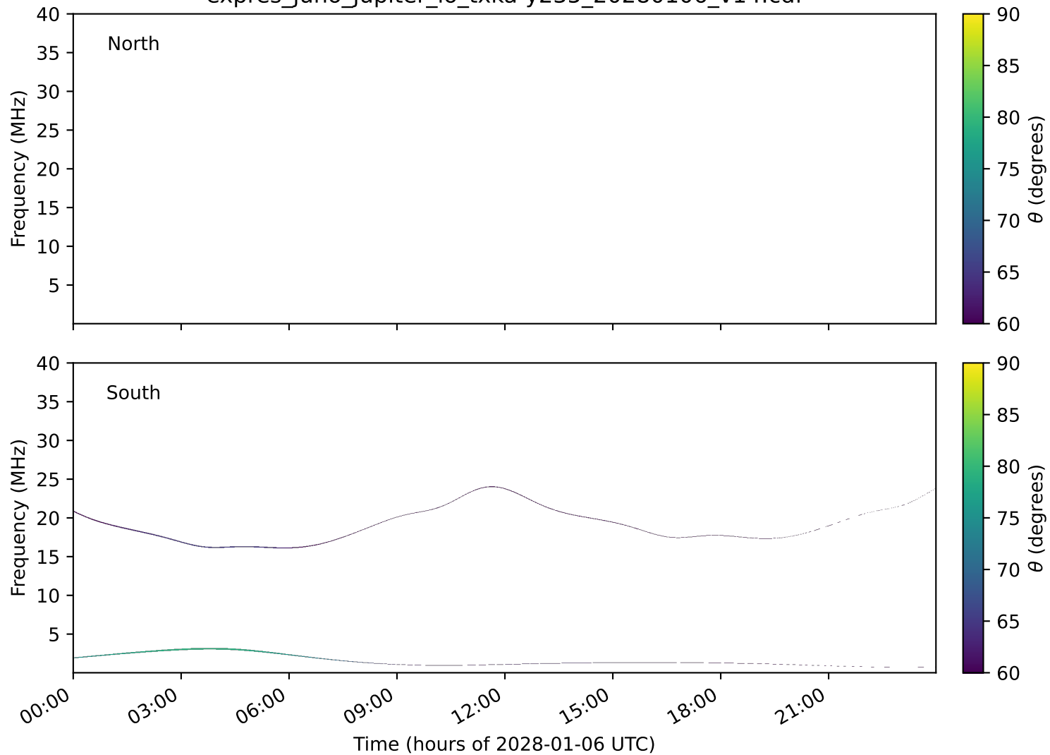
expres_juno_jupiter_io_txka-y235_20280106_v14.cdf
