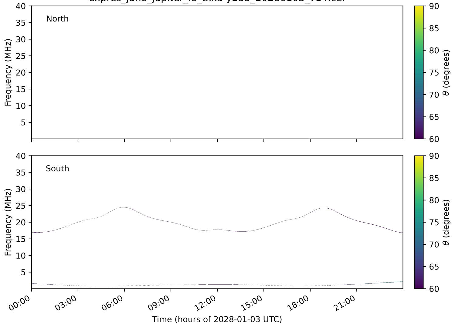
expres_juno_jupiter_io_txka-y235_20280103_v14.cdf
