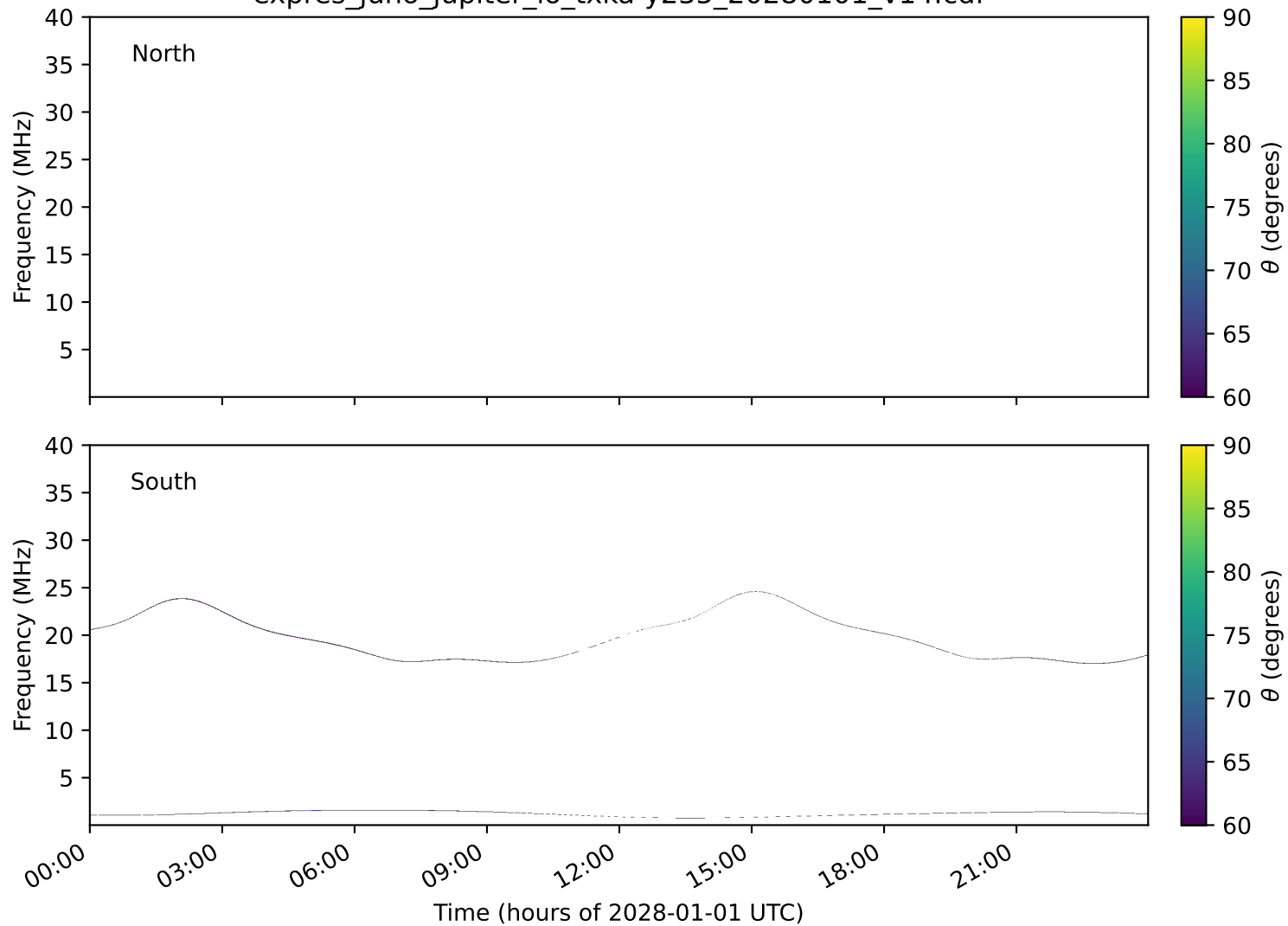
expres_juno_jupiter_io_txka-y235_20280101_v14.cdf
