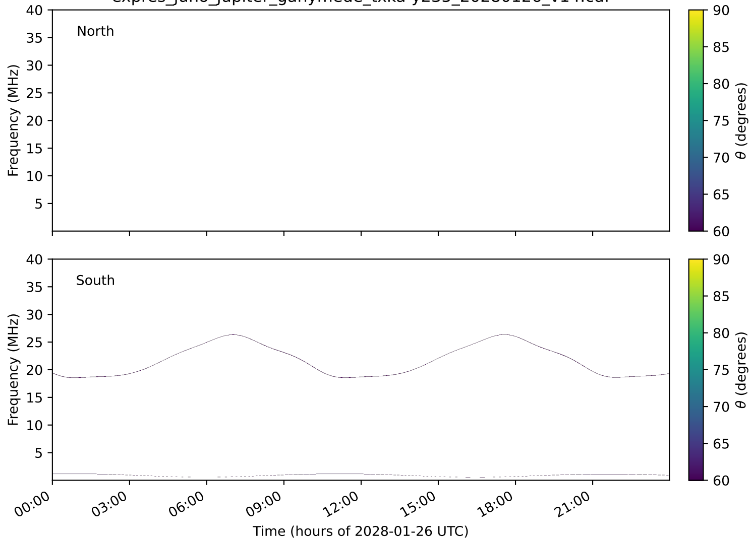
expres_juno_jupiter_ganymede_txka-y235_20280126_v14.cdf
