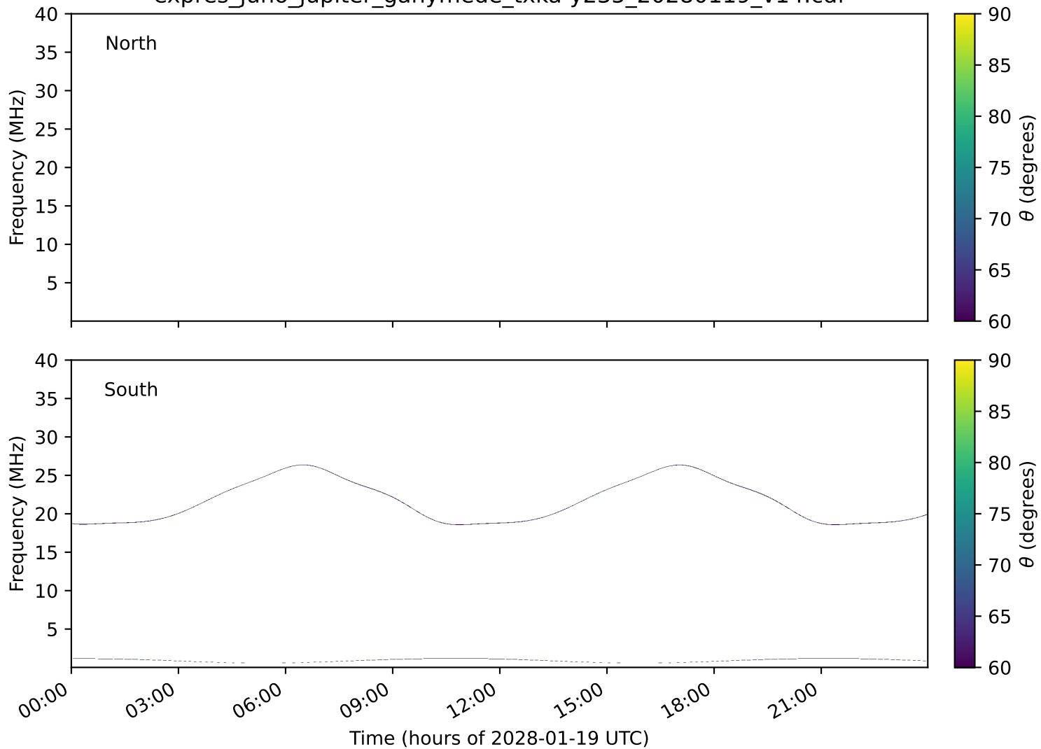
expres_juno_jupiter_ganymede_txka-y235_20280119_v14.cdf
