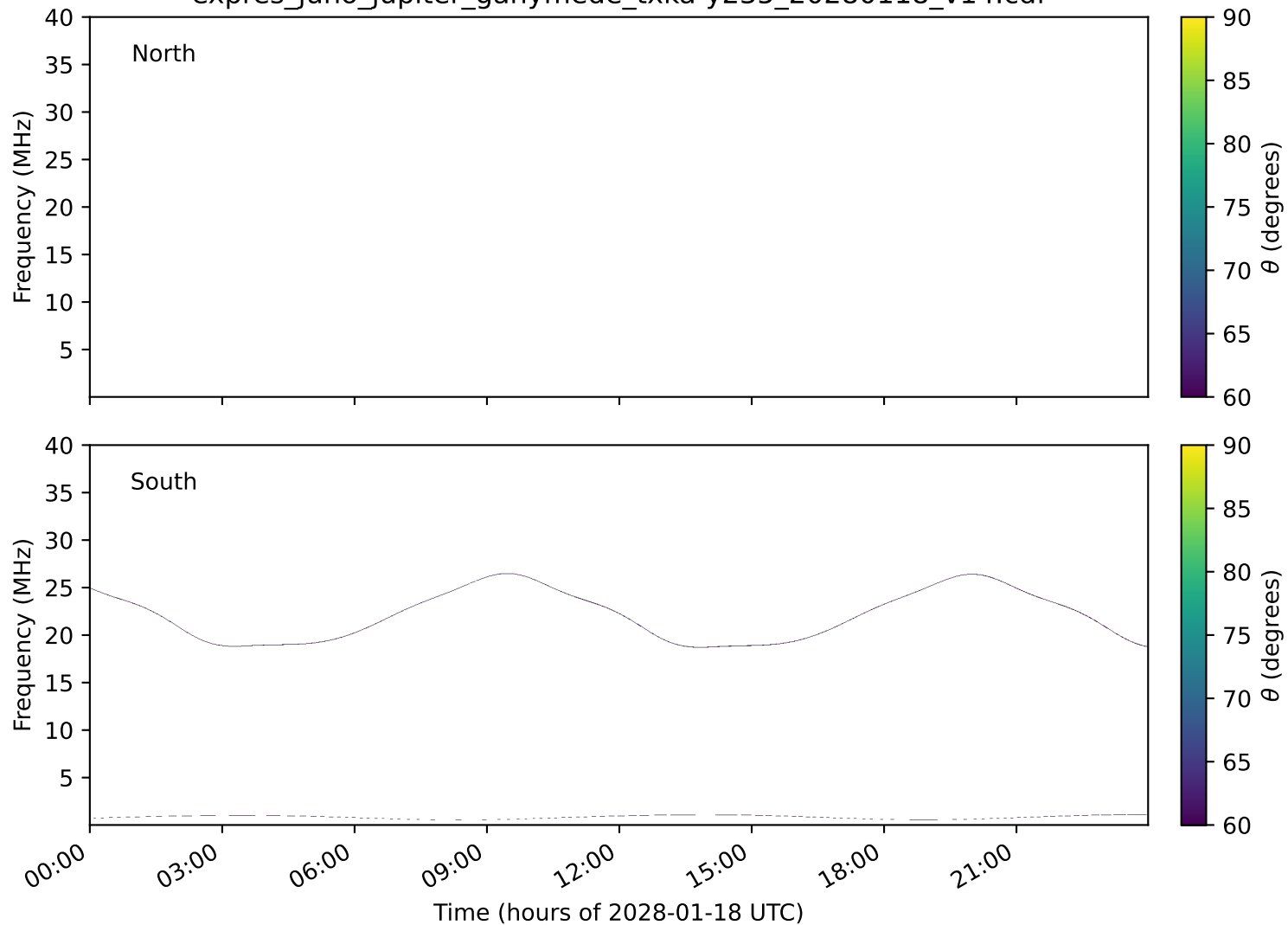
expres_juno_jupiter_ganymede_txka-y235_20280118_v14.cdf
