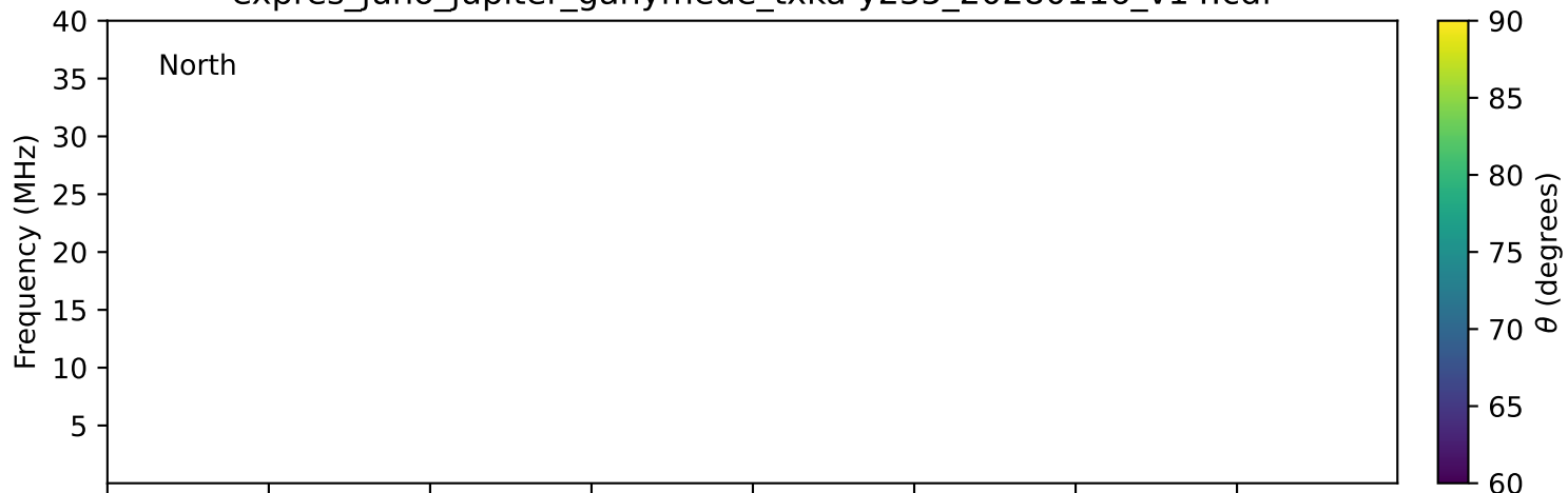
expres_juno_jupiter_ganymede_txka-y235_20280116_v14.cdf
