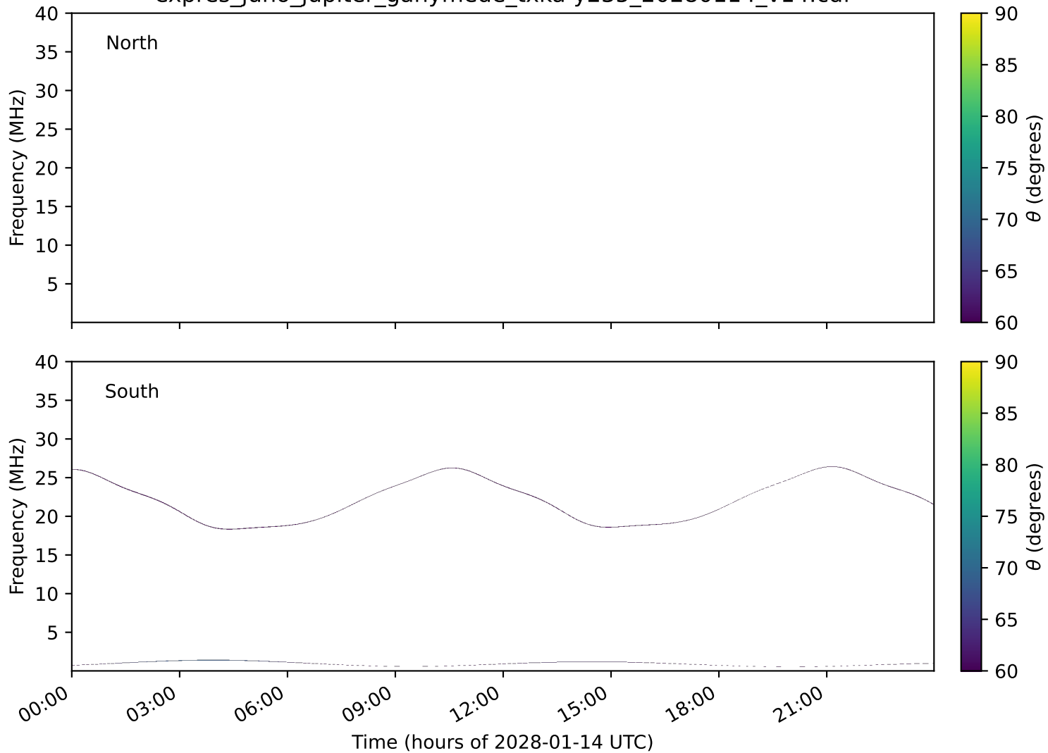
expres_juno_jupiter_ganymede_txka-y235_20280114_v14.cdf
