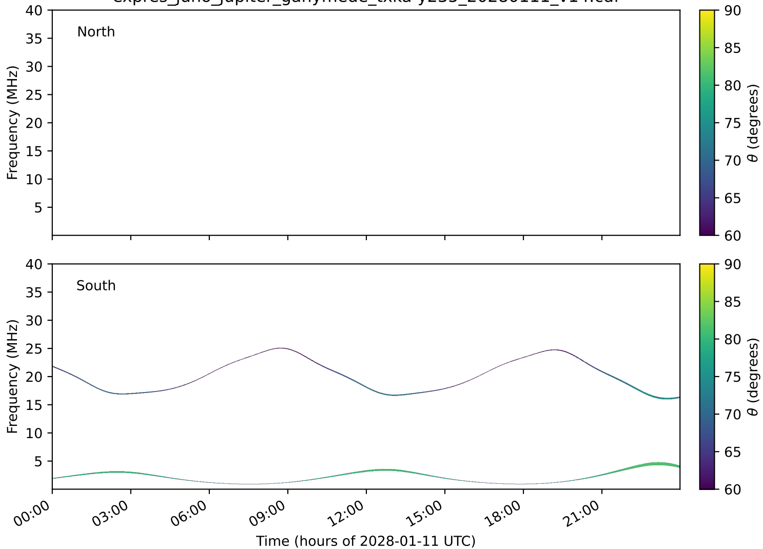
expres_juno_jupiter_ganymede_txka-y235_20280111_v14.cdf
