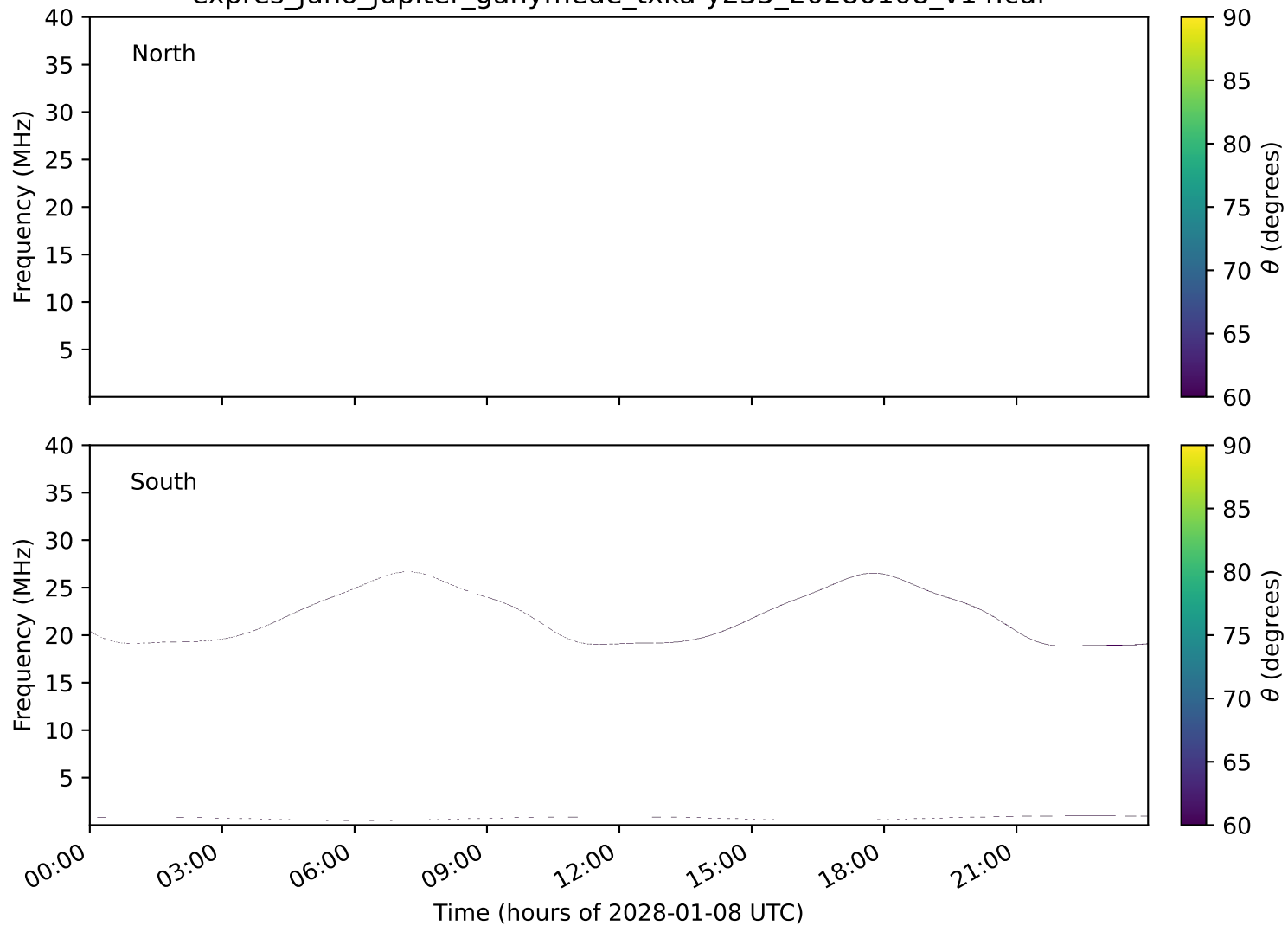
expres_juno_jupiter_ganymede_txka-y235_20280108_v14.cdf
