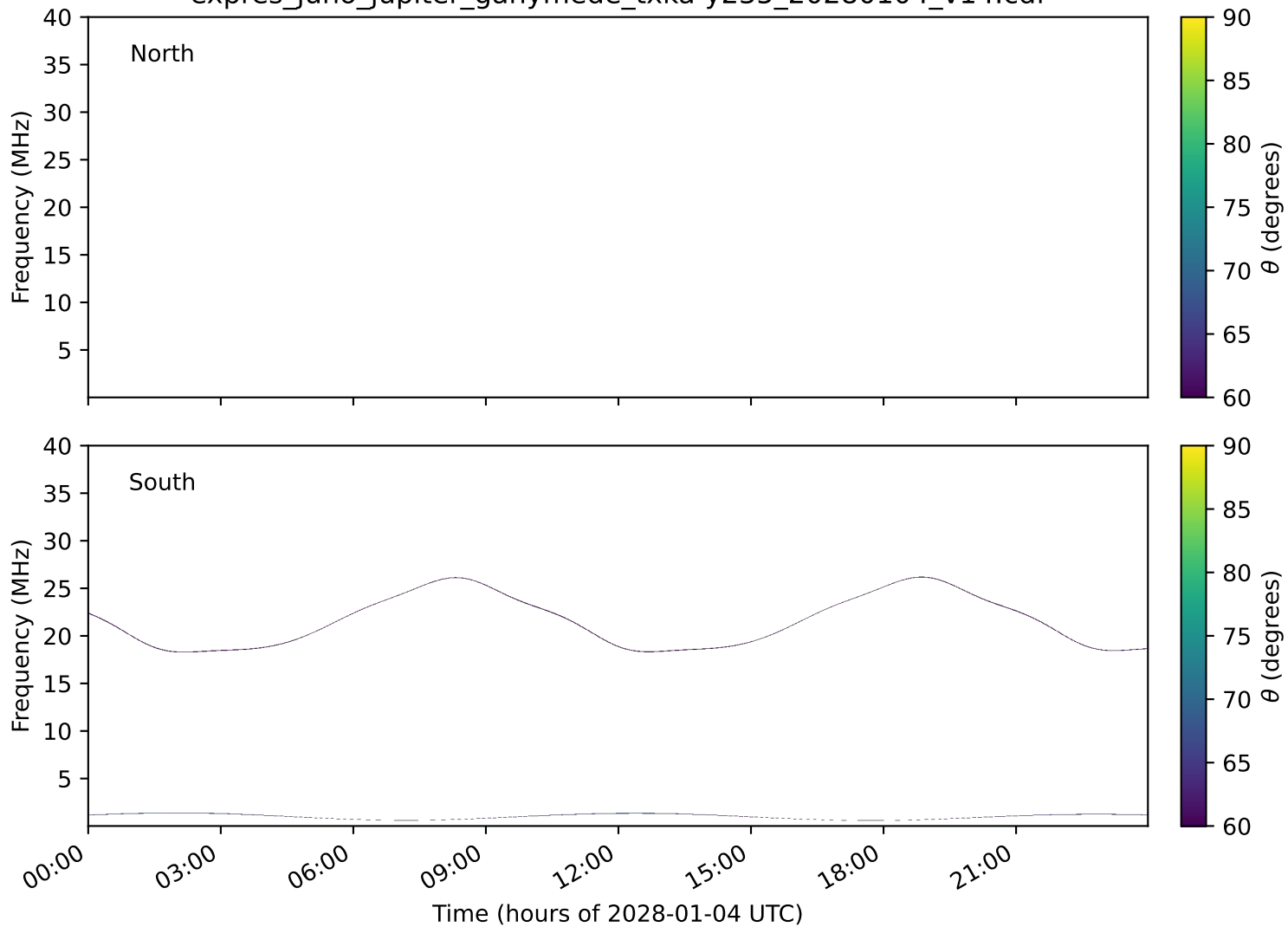
expres_juno_jupiter_ganymede_txka-y235_20280104_v14.cdf
