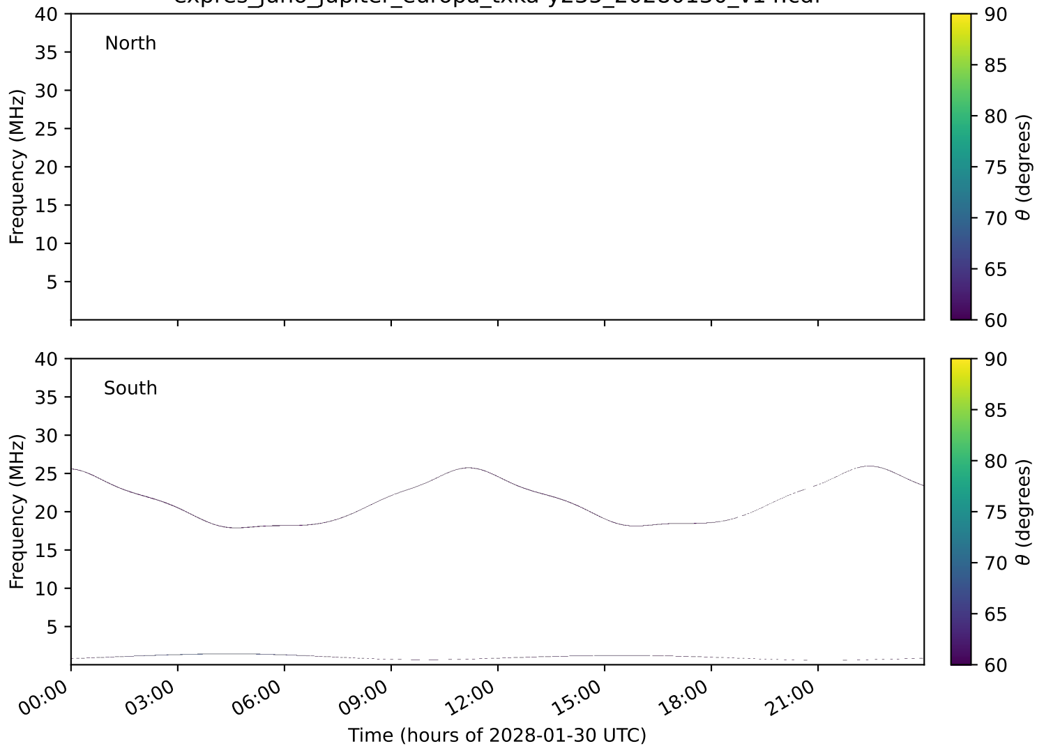
expres_juno_jupiter_europa_txka-y235_20280130_v14.cdf
