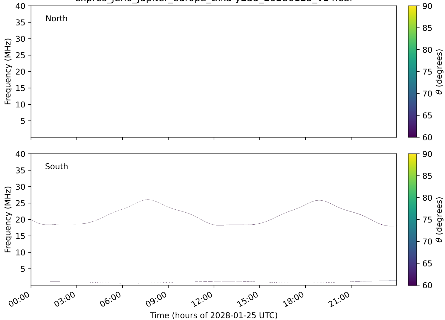
expres_juno_jupiter_europa_txka-y235_20280125_v14.cdf
