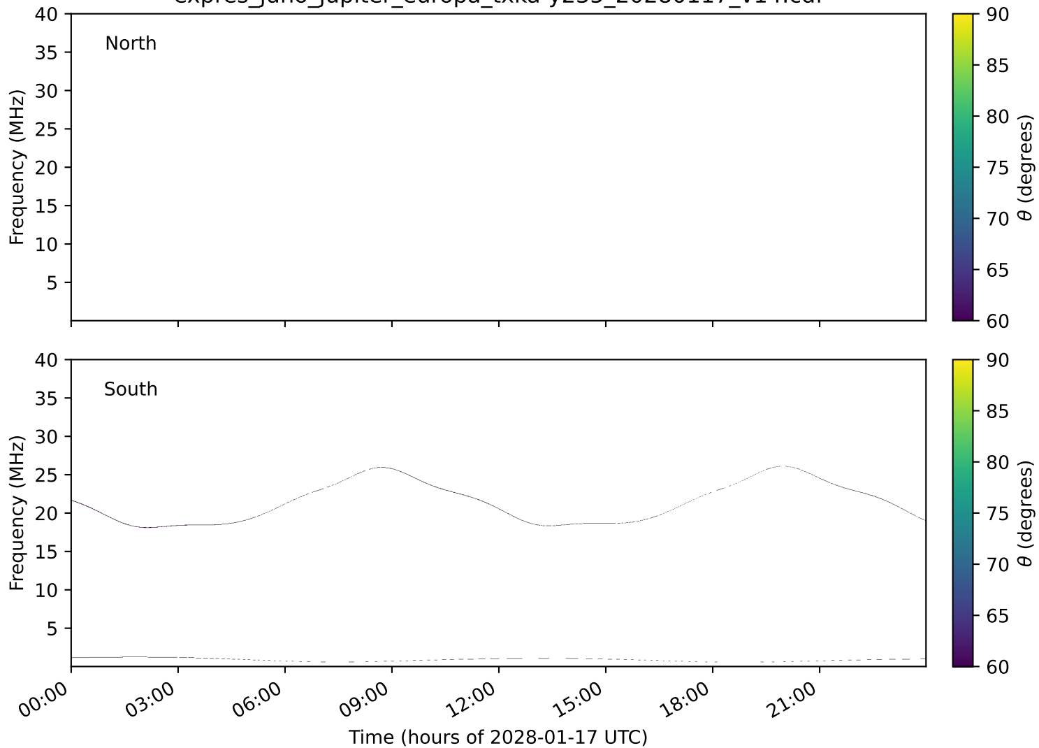
expres_juno_jupiter_europa_txka-y235_20280117_v14.cdf
