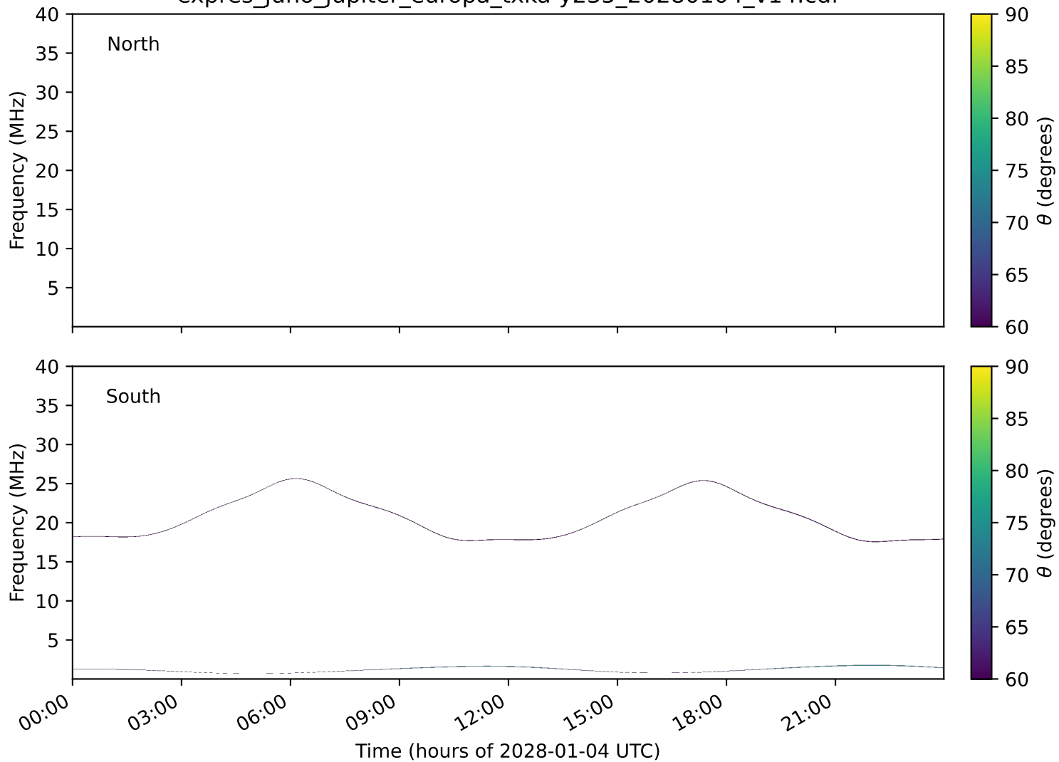
expres_juno_jupiter_europa_txka-y235_20280104_v14.cdf
