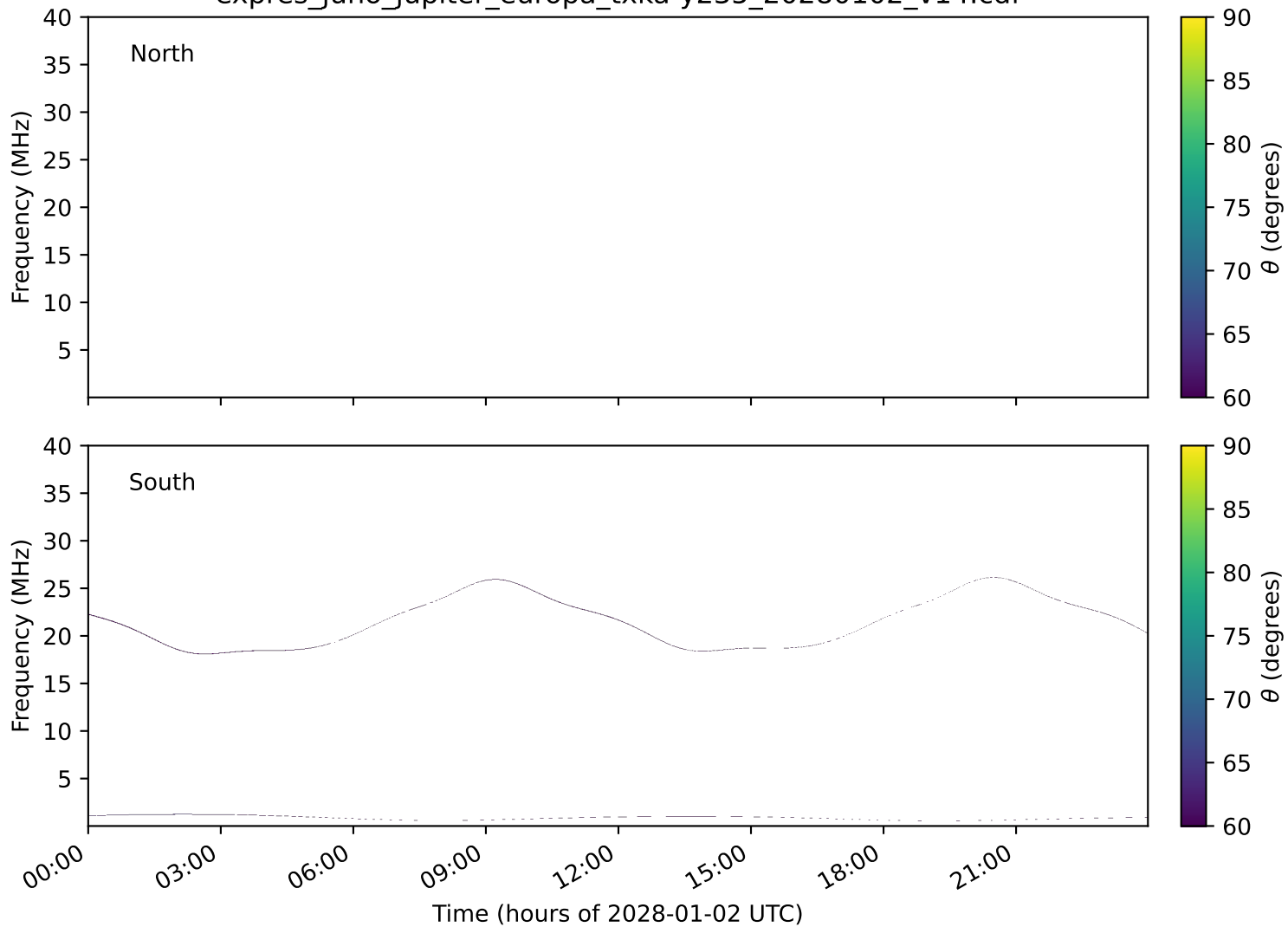
expres_juno_jupiter_europa_txka-y235_20280102_v14.cdf
