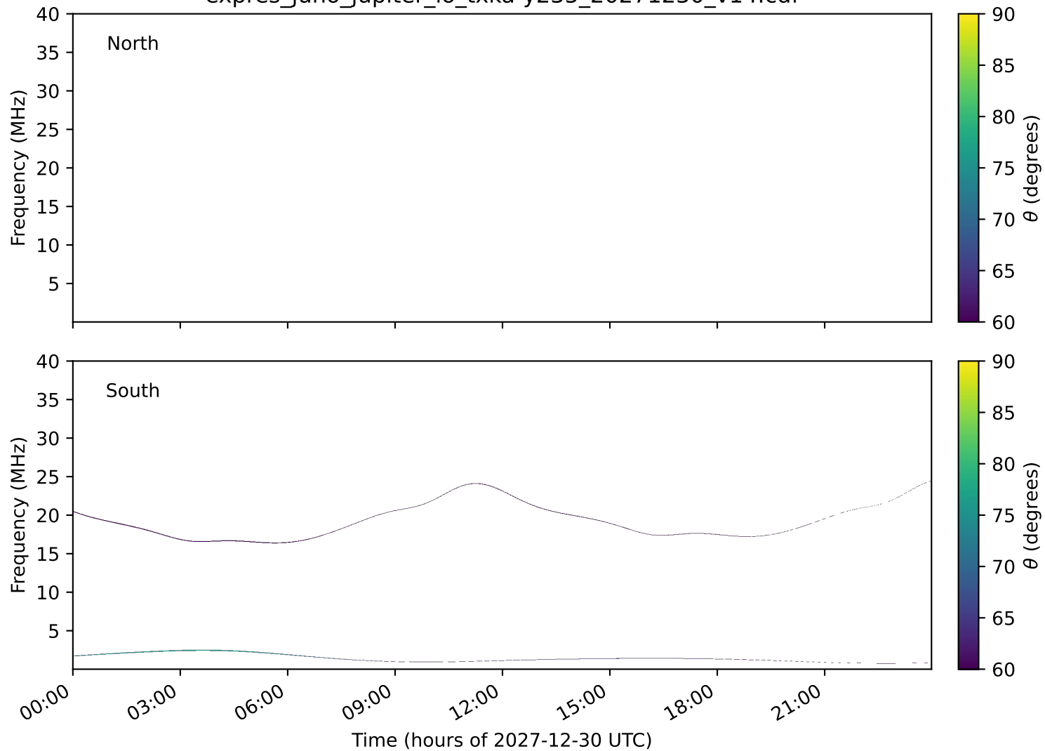
expres_juno_jupiter_io_txka-y235_20271230_v14.cdf
