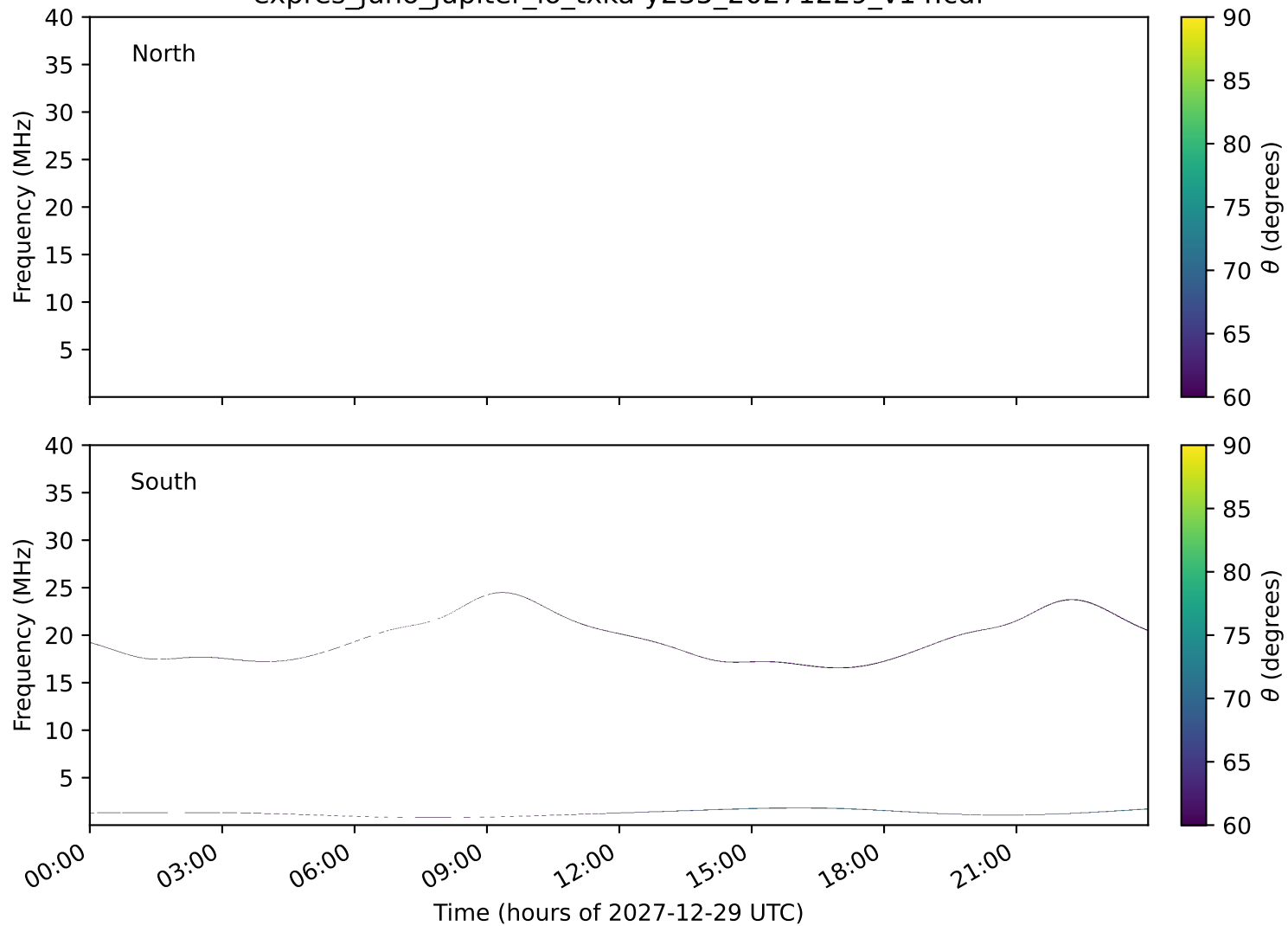
expres_juno_jupiter_io_txka-y235_20271229_v14.cdf
