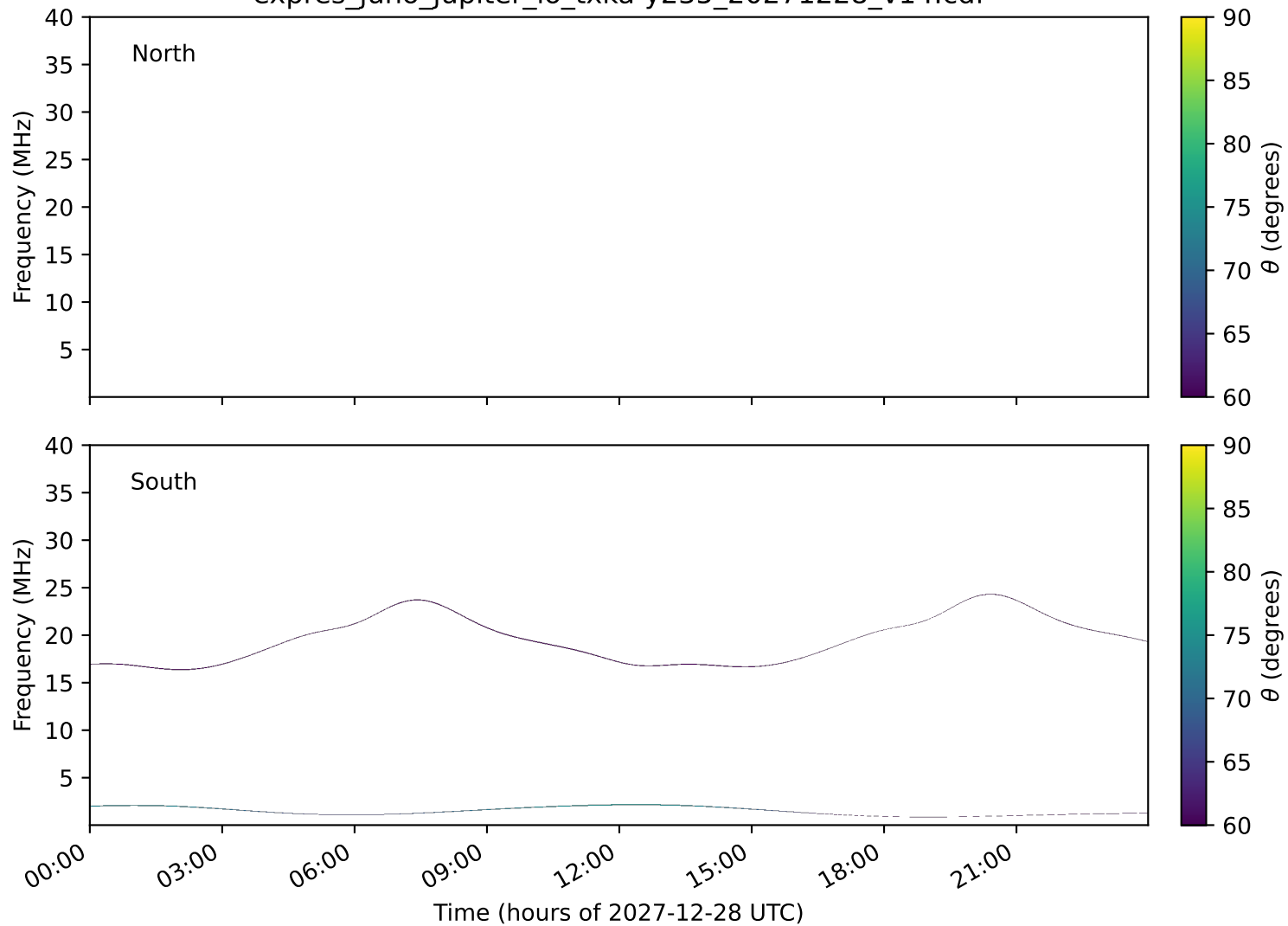
expres_juno_jupiter_io_txka-y235_20271228_v14.cdf
