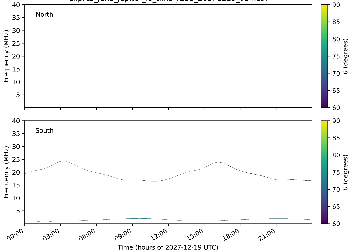
expres_juno_jupiter_io_txka-y235_20271219_v14.cdf
