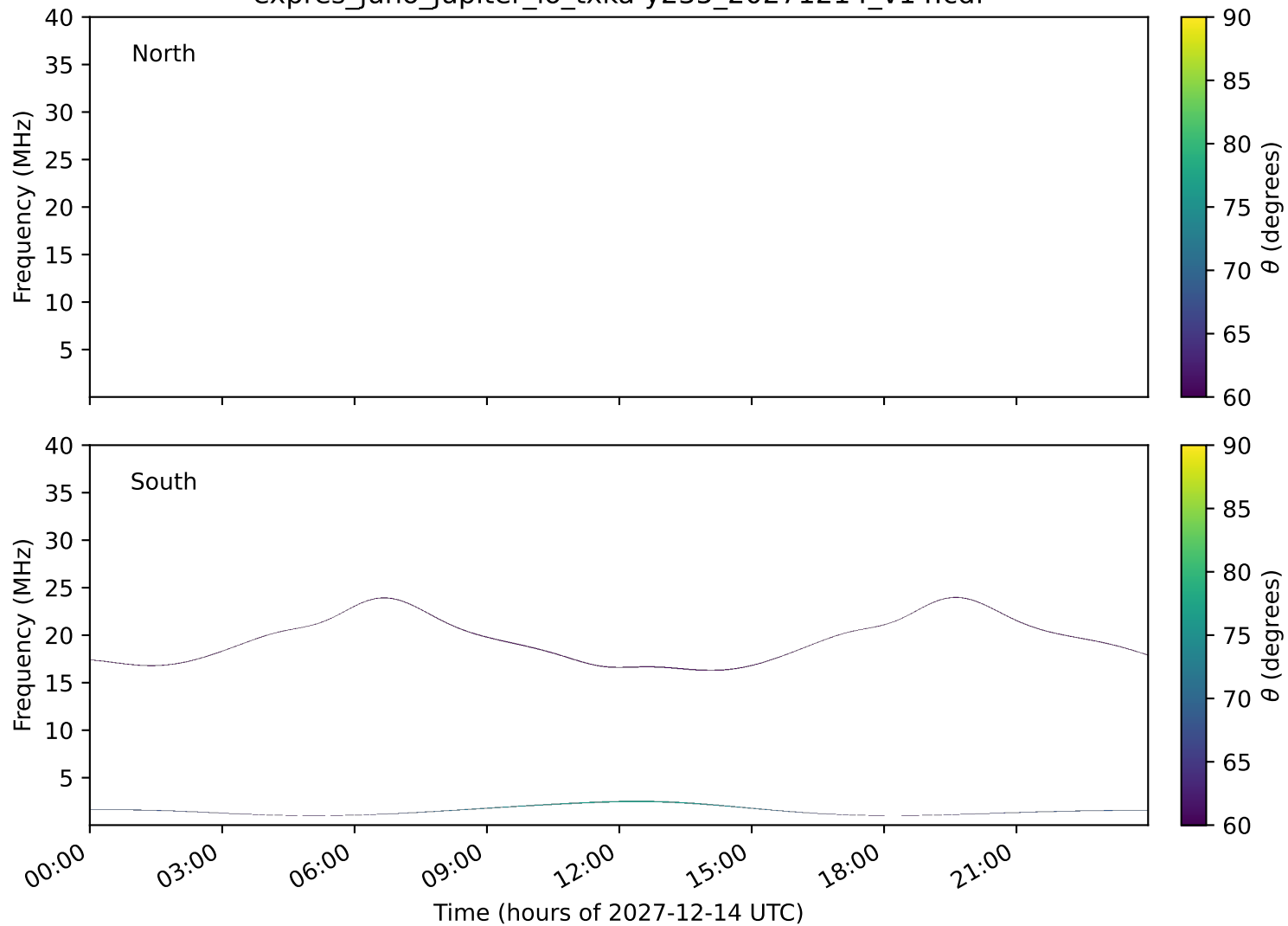
expres_juno_jupiter_io_txka-y235_20271214_v14.cdf
