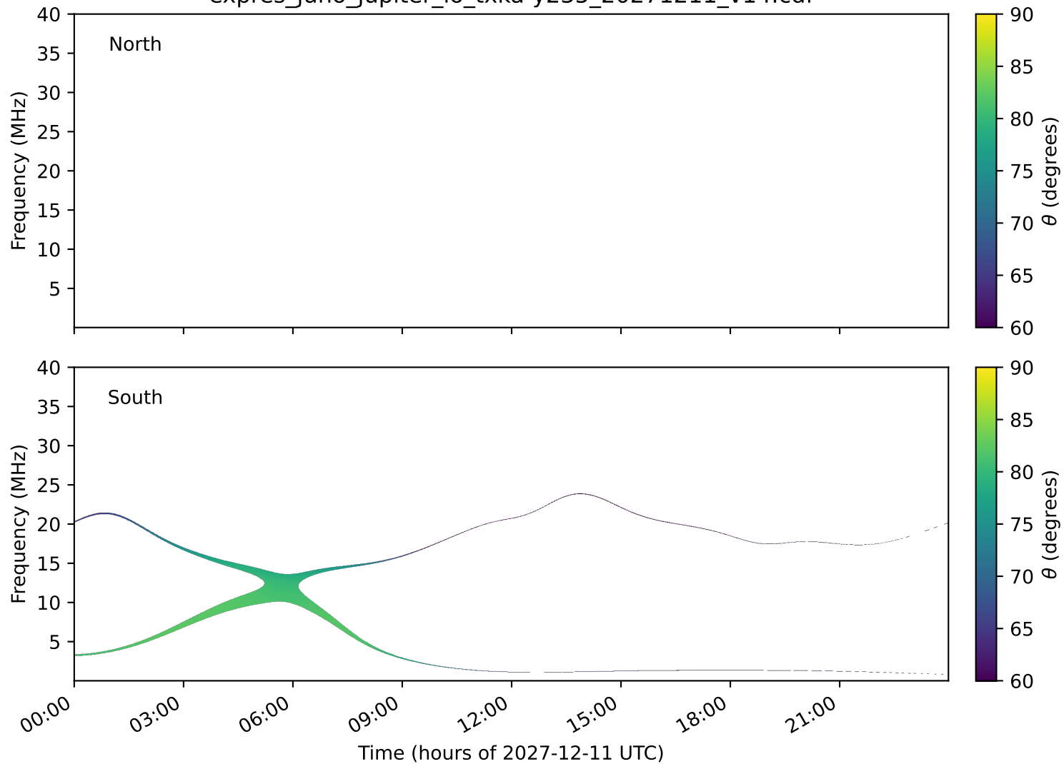
expres_juno_jupiter_io_txka-y235_20271211_v14.cdf
