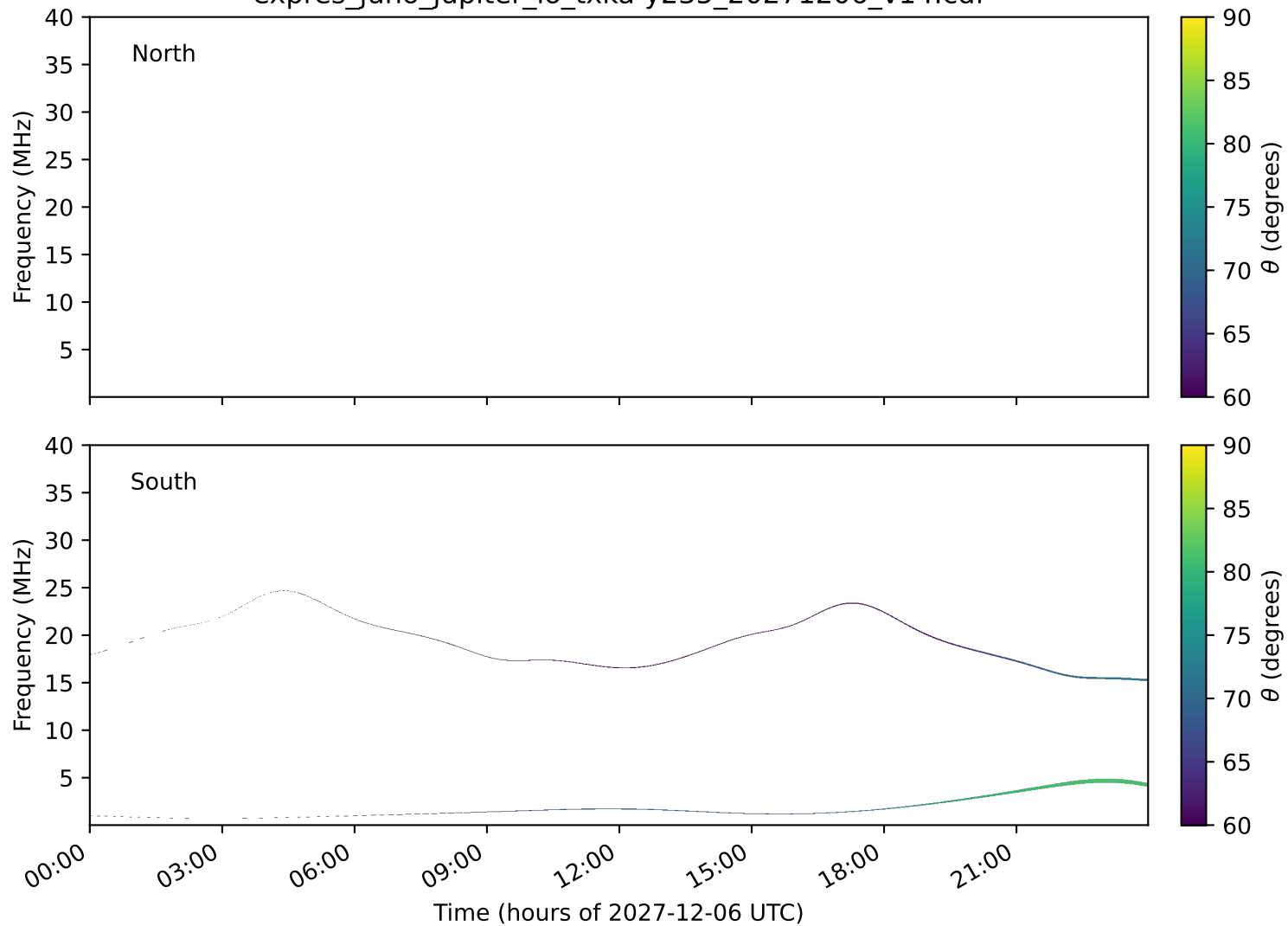
expres_juno_jupiter_io_txka-y235_20271206_v14.cdf
