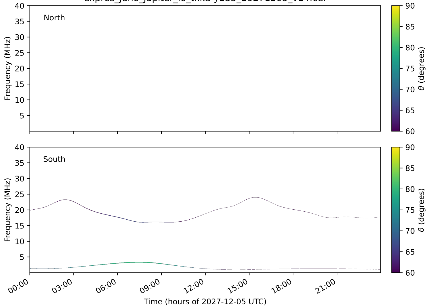
expres_juno_jupiter_io_txka-y235_20271205_v14.cdf
