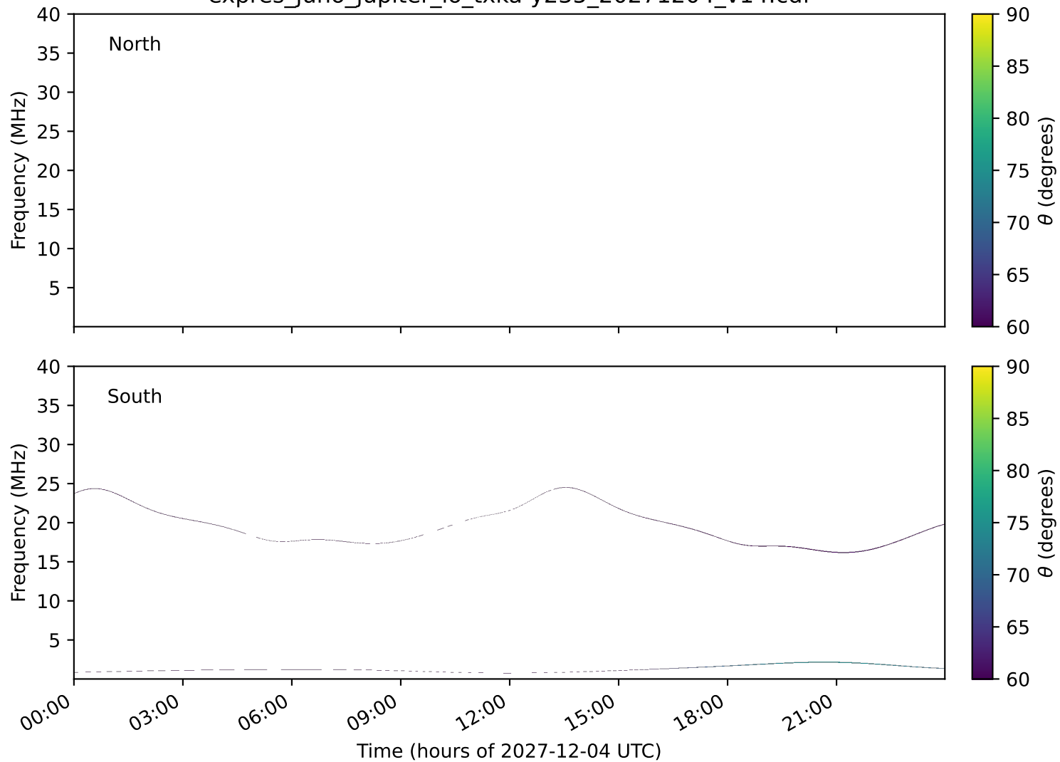
expres_juno_jupiter_io_txka-y235_20271204_v14.cdf
