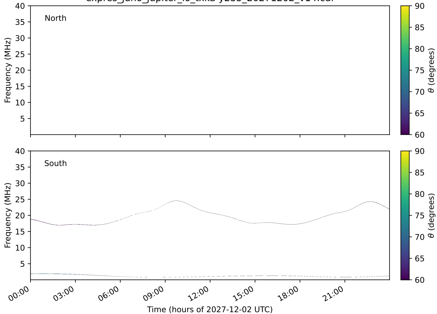
expres_juno_jupiter_io_txka-y235_20271202_v14.cdf
